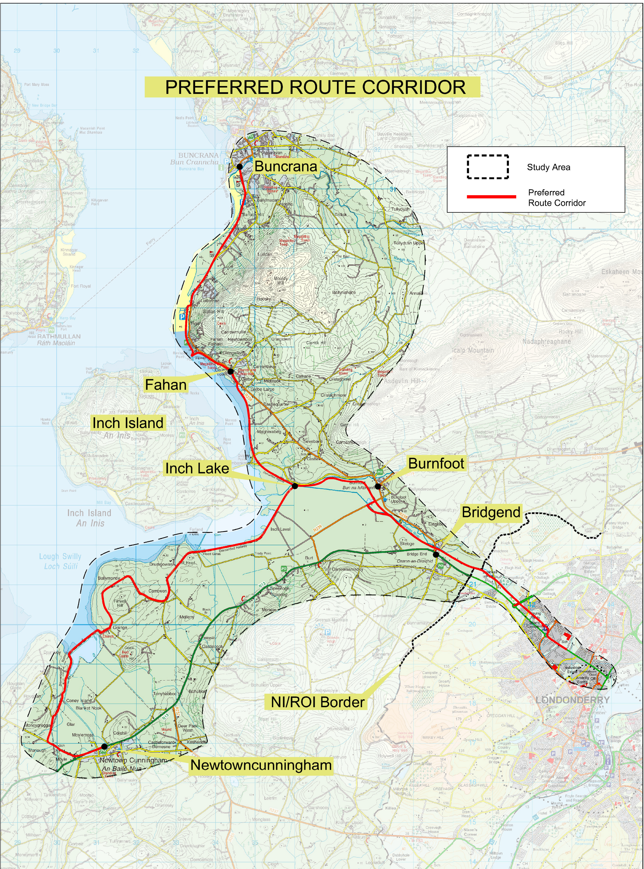
NORTH WEST GREENWAY NETWORK Route 1 - Preferred Route Corridor Selection Report Figure 8.9.1 - Preferred Route Corridor
